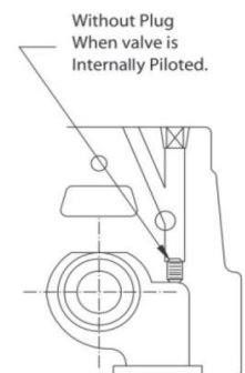
Section Y-Y
